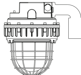
Lamp Post Mount 90° (suffix PM90)
