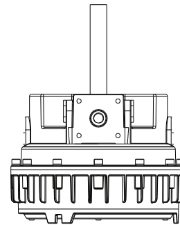
Pendant Mount (suffix PM)
